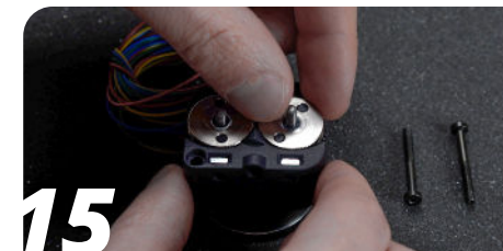
15 With the lever in the leftmost position, insert the drivegears
