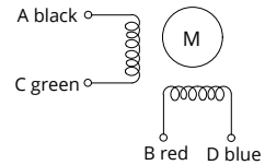
Wiring Diagram
